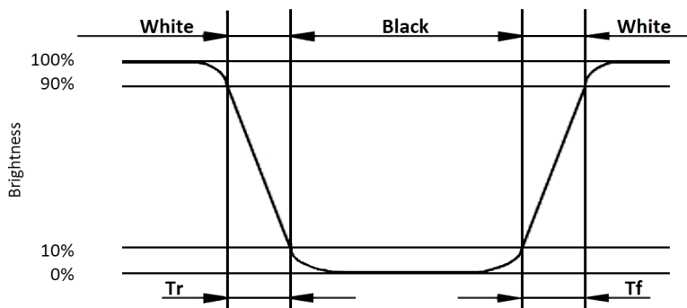
Figure 6: Response Times
